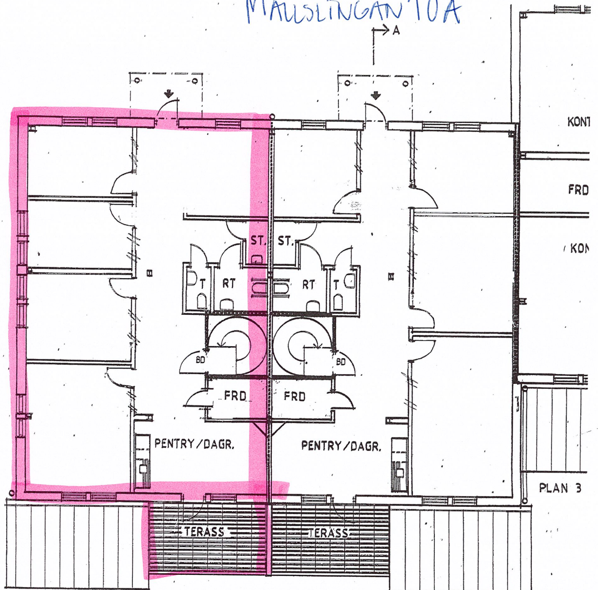
PLAN 3
