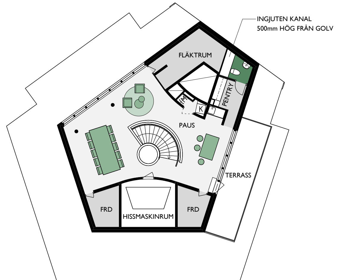
PLAN 21, 11 tr 88 KVM
