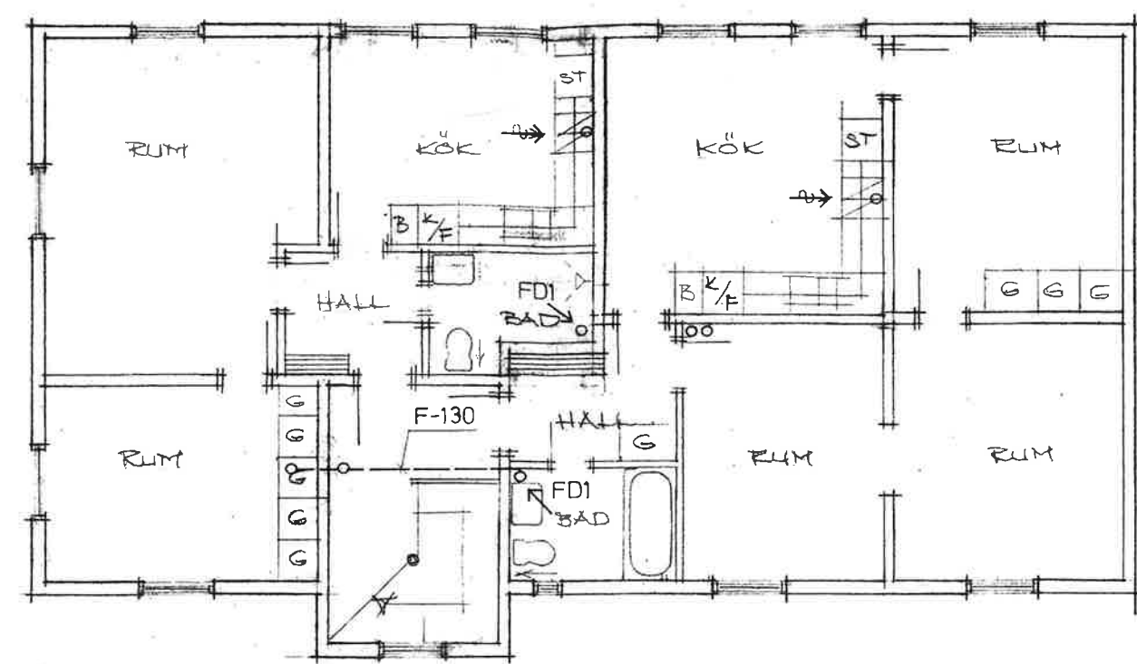
PLAN 1 TR.
