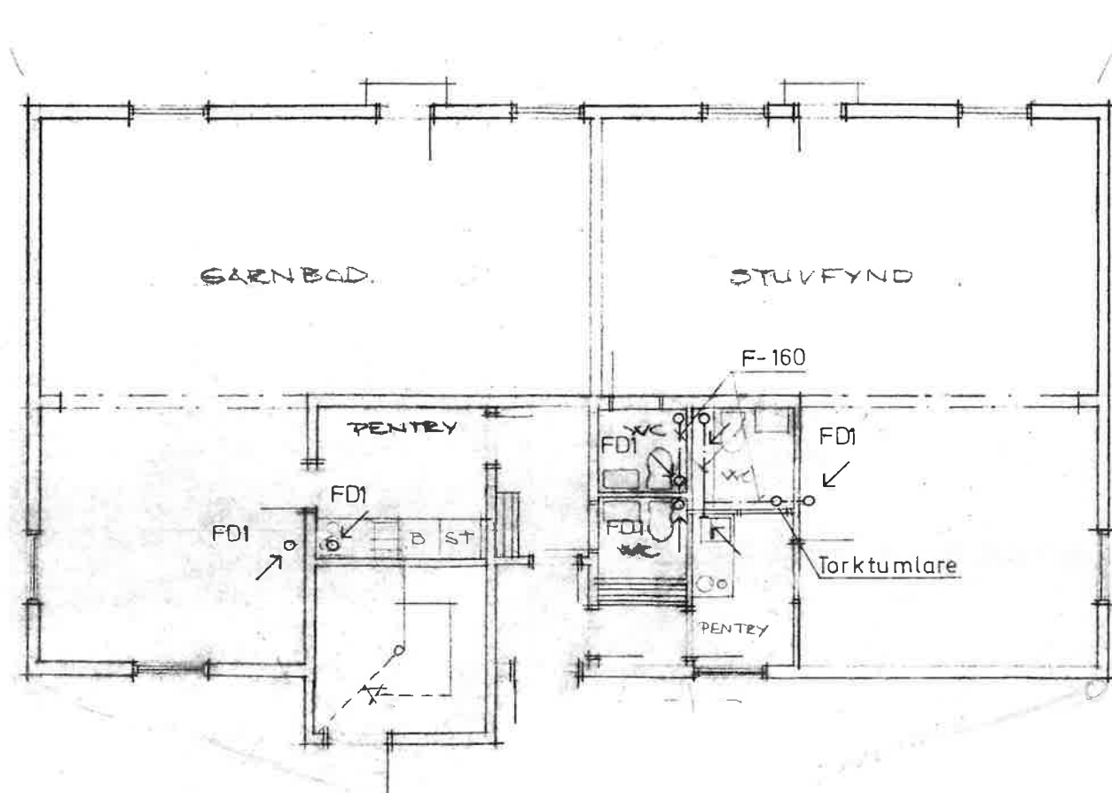
BOTTEN PLAN
